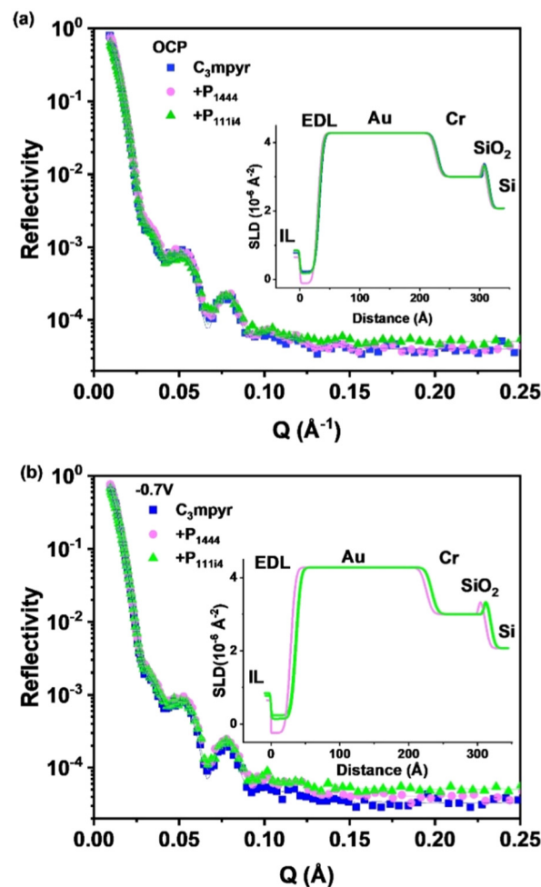
Fig. 5 Neutron reflectometry curves for electrolytes/electrode interfaces for (a) 0 V; (b) -0.7 V vs. OCP. Solid lines are fitting curves with four-slab model with varied parameters only for EDL. Insets are SLD profiles.
