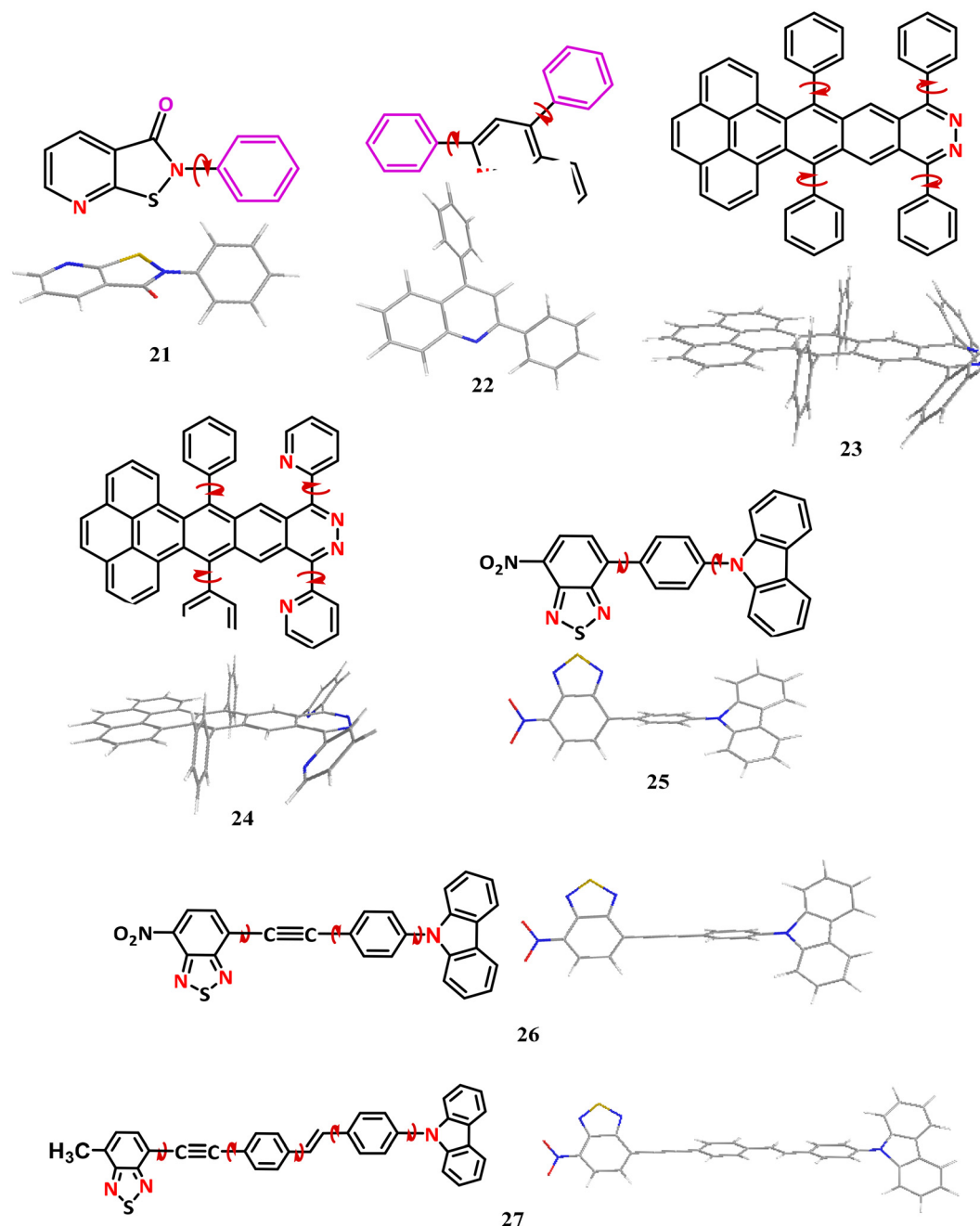
Fig. 7 Examples of AIEgens developed from the decoration of ACQphores with aromatic rotors.
