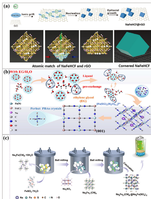
Fig. 2 Schematic illustration of NaFeHCF@rGO synthesis and structural diagrams of cubic and cornered NaFeHCF (a). Reproduced with permission. Copyright 2024, Wiley. 28 Schematic of the synthesis of PB-EGs via the ligand pre-exchange strategy (b). Reproduced with permission. Copyright 2025, Royal Society of Chemistry. 29 Schematic illustration of the synthesis of an NFS@Fe-PB sample based on the mechanochemical ball milling strategy (c). Reproduced with permission. Copyright 2025, Wiley. 30
