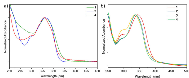
Fig. 3 UV-Vis spectra of (a) complexes 1 , 2 and 4 in DCM and (b) complexes 1–4 in a mixture of DMEM (Dulbecco's modified Eagle's medium, [4.5 g L −1 D-Glucose, L-Glutamin, [4.5 g L −1 Pyruvat, Gibco™) and DMSO (dimethylsulfoxide) in a 15 : 1 ratio.
