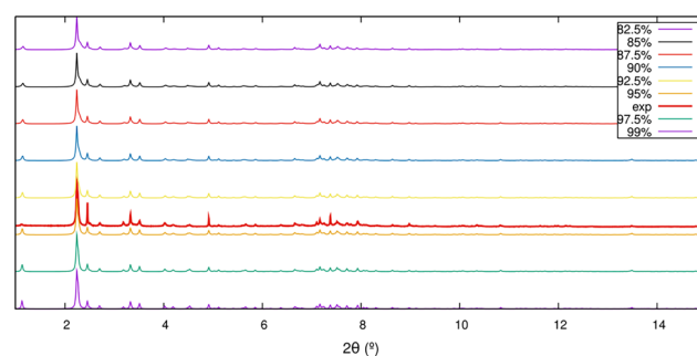
Fig. 7 DIFFaX simulated XRD patterns ( \lambda = 0.49587 Å) for UWY -ECNU-13A intergrowths at high UWY proportions (thin traces, from bottom to top the UWY content is 99, 97.5, 95, 92.5, 90, 87.5, 85 and 82.5%). The thick red trace corresponds to the experimental SPXRD. For the whole UWY -ECNU-13A range, please check Fig. S6.†
