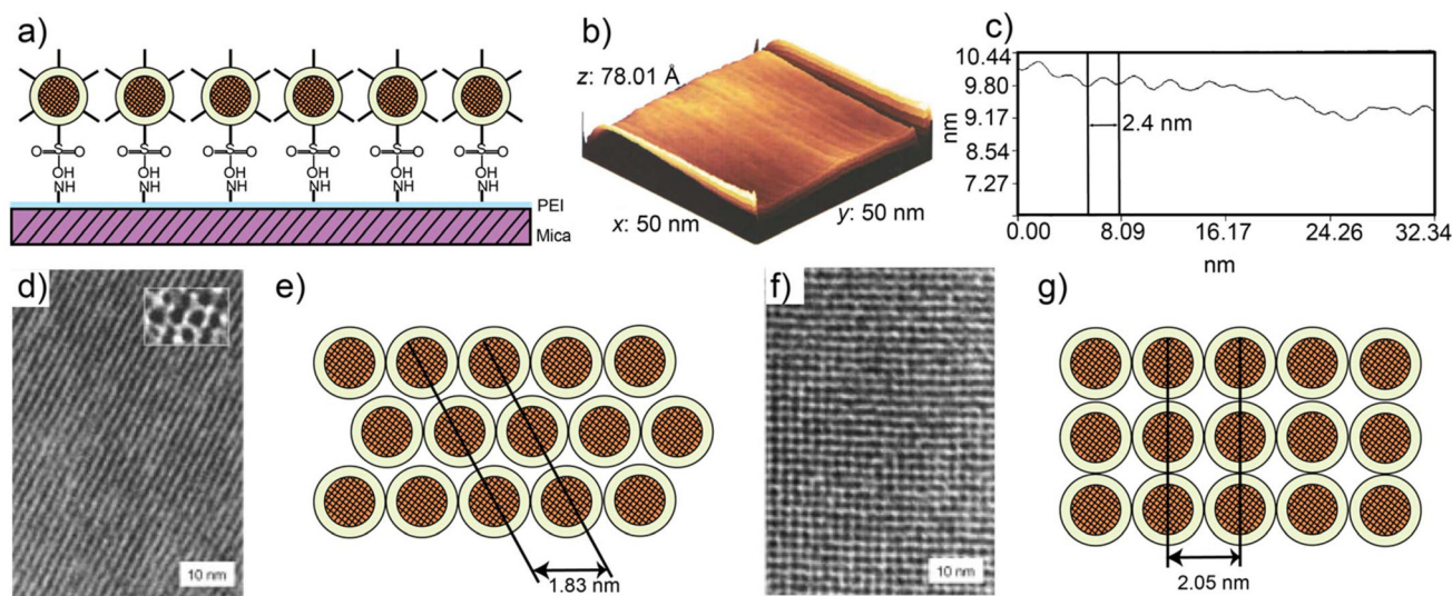
Fig. 2 Self-assembled monolayer arrays of NCs on substrates. (a) Schematic illustration of \text{Au}_{55}(\text{Ph}_2\text{PC}_6\text{H}_4\text{SO}_3\text{H})_{12}\text{Cl}_6 NC on PEI-coated mica substrate. (b and c) AFM image of monolayer film and corresponding height profile. Reproduced with permission from ref. 91 Copyright © 1995 Wiley-VCH. (d) TEM image showing a hexagonally close-packed array of [\text{Au}_{55}(\text{Ph}_2\text{PC}_6\text{H}_4\text{SO}_3\text{H})_{12}\text{Cl}_6] NC on carbon substrate. (e) Schematic illustration of hcp arrays of NCs. (f) TEM image showing a cubic close packed array of [\text{Au}_{55}(\text{Ph}_2\text{PC}_6\text{H}_4\text{SO}_3\text{H})_{12}\text{Cl}_6] NC on carbon substrate. (g) Schematic illustration of ccp arrays of NCs. Reproduced with permission from ref. 92 Copyright © 2000 Wiley-VCH.
