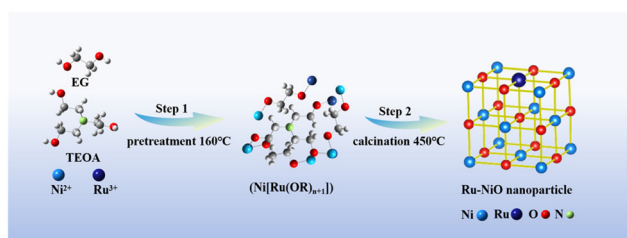
Scheme 1 Synthesis of 3% Ru-doped NiO nanoparticles achieved through a two-step thermal treatment method.
