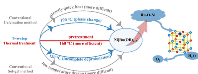
Scheme 2 Synthetic reaction mechanism of different methods for the substitution of Ru for Ni in the NiO lattice.
