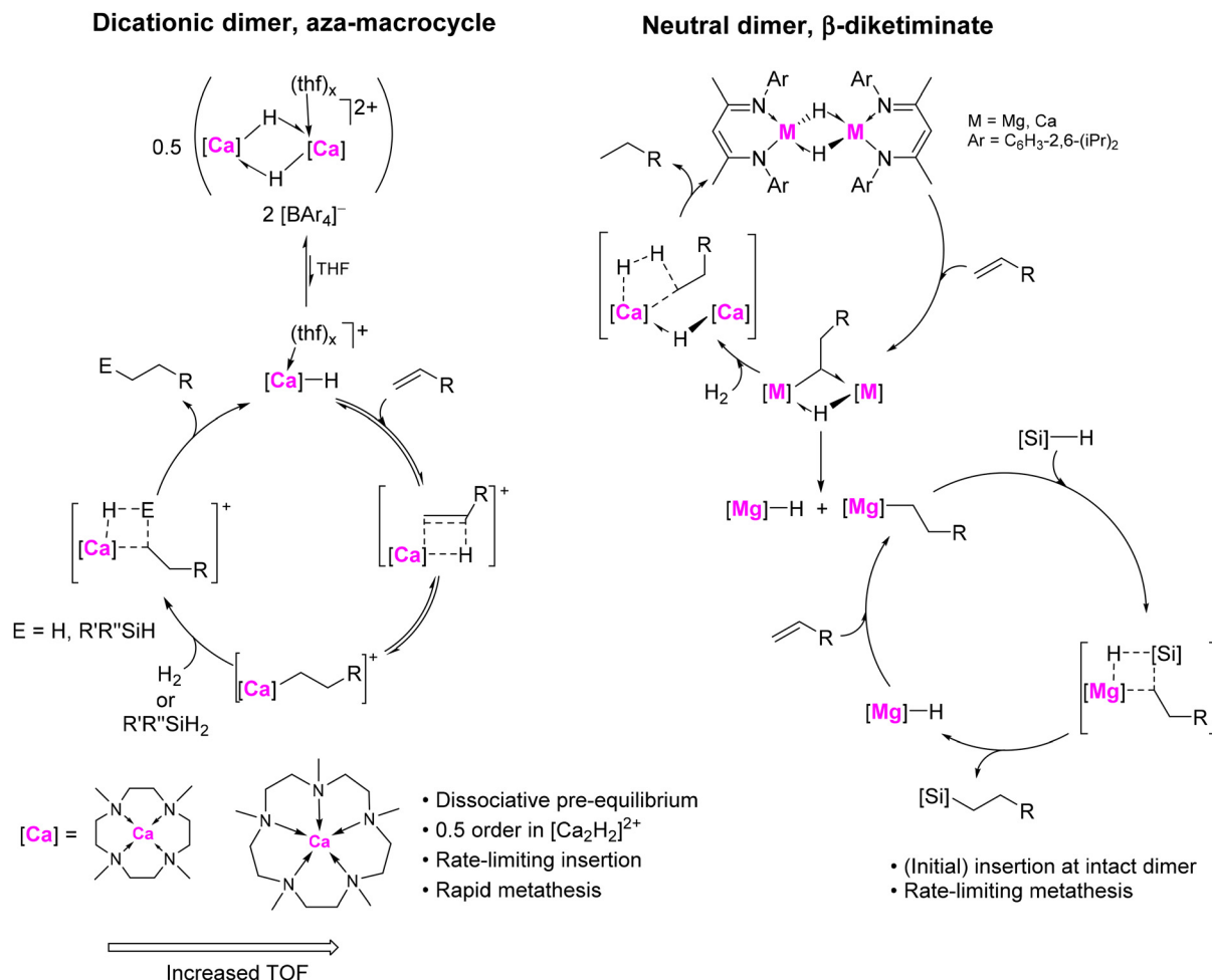
Scheme 20 Contrast in proposed mechanisms for olefin hydrogenation and hydrosilylation mediated by Me 4 TACD/Me 5 PACP-calcium and BDI dipp -calcium/magnesium catalysts.
