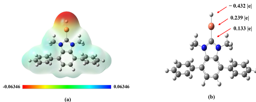
Fig. 2 (a) ESP surface map of NHC-Cu(I)-H. (b) The cluster model of NHC-Cu(I)-H showing NBO charges.
