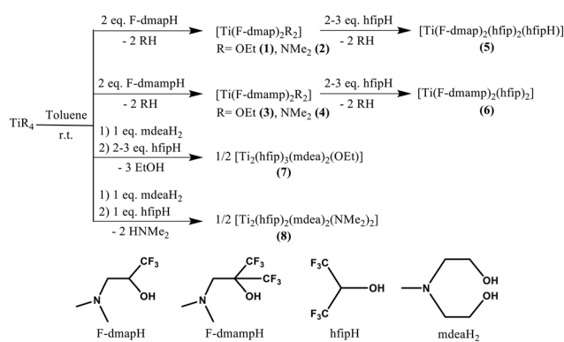
Scheme 1 Synthesis of new heteroleptic Ti(IV) aminofluoroalkoxides 1–8.
