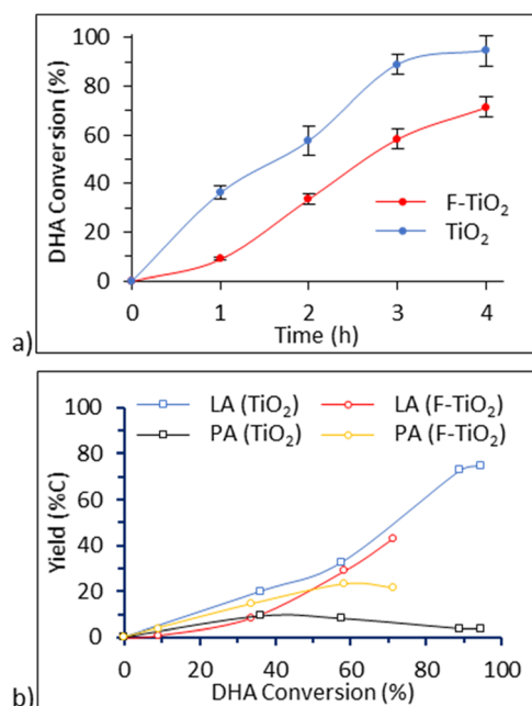
Fig. 11 a) DHA conversion catalyzed by undoped \text{TiO}_2 and F-doped \text{TiO}_2 catalyst C-3 and b) evolution of obtained products' yields (%) as a function of the DHA conversion. Reaction conditions: 25 mg catalyst; DHA = 0.5 \text{ g L}^{-1} ; T = 120^\circ\text{C} ; duration = 4 h; 6 bar argon.
