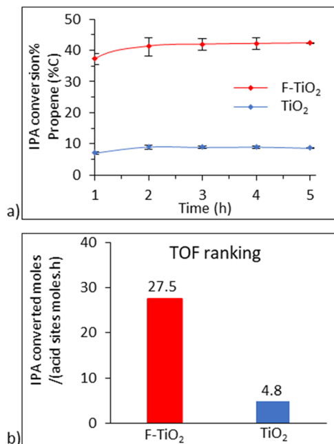
Fig. 10 Isopropanol reactions performed over undoped \text{TiO}_2 and F-doped \text{TiO}_2 catalyst C-3: a) evolution of propene yields with time, and b) TOF values. Reaction conditions: 80 mg catalyst; total flow rate = 5 \text{ L h}^{-1} (1% IPA in \text{N}_2 ); T = 200^\circ\text{C} ; time on stream = 5 h.
