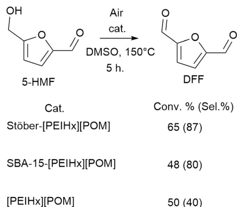
Scheme 3 Direct oxidation of 5-HMF catalysed by SiO 2 -[PEIH] x [PMO]. Reaction conditions: 140 mg of 5-HMF (1.11 mmol), 22.5 mg of SBA-15-[PEIH] x [PMO 12 O 40 ] (0.06 mol% [PMO 12 O 40 ], 0.7 mol% Mo), 22.5 mg of Stöber-[PEIH] x [PMO 12 O 40 ] (0.05 mol%, PMO 12 O 40 , 0.6 mol% Mo) or 1.2 mg of [PEIH] x [PMO 12 O 40 ] (0.05 mol%, PMO 12 O 40 , 0.6 mol% Mo), 6 mL of solvent, 65 mg of naphthalene as the internal standard. Conversion and selectivity were determined by GC-FID.
