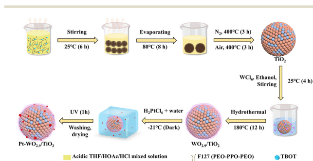
Scheme 1 Schematic of the synthesis of TiO 2 microspheres, WO 2.9 /TiO 2 , and Pt-WO 2.9 /TiO 2 photocatalyst.
