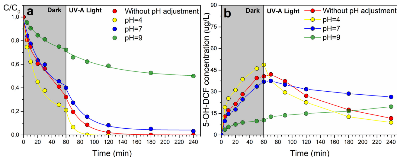
Fig. 10 Effect of pH on catalytic and photocatalytic degradation of diclofenac using Cu/2Ti8Mn-HT catalyst: (a) normalized kinetic curves of diclofenac degradation; (b) concentration trend of 5-OH-DCF, both in dark and light conditions.
