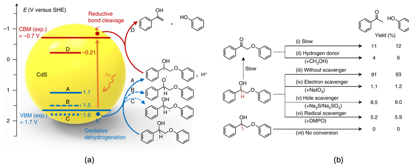
Scheme 2 (a) Proposed electron-hole coupled (EHCO) mechanism for CdS-catalysed C_{\beta} -O bond cleavage of a dimeric \beta -O-4 lignin model compound through a C_{\alpha} radical intermediate; (b) the control experiments with various reactants or additives (this scheme has been reproduced from ref. 22 with permission from Nature Publication Group, copyright 2018).
