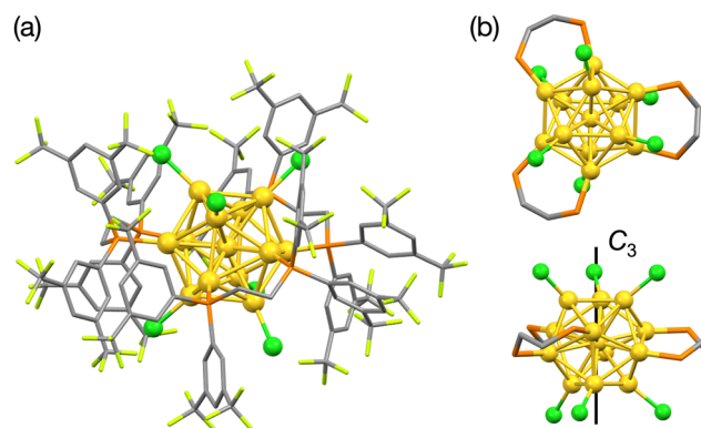
Fig. 2 (a) The entire structure of \text{Au}_{13}:\text{dppeF} , as determined by SCXRD analysis. (b) Top and side views of \text{Au}_{13}:\text{dppeF} . Hydrogen atoms, \text{ArF} moieties, a solvent molecule, and the \text{PPh}_4^+ ion are omitted for clarity. Color code: Au, yellow; P, orange; Cl, green; C, gray; F, yellow-green.
