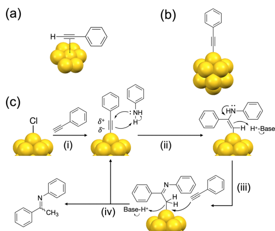
Fig. 5 Schematic representation of (a) π-ligation of PA-H to an Au surface and (b) σ-bonding of PA to Au NC. (c) Proposed reaction mechanism of hydroamination of PA-H on Au 13 NCs.
