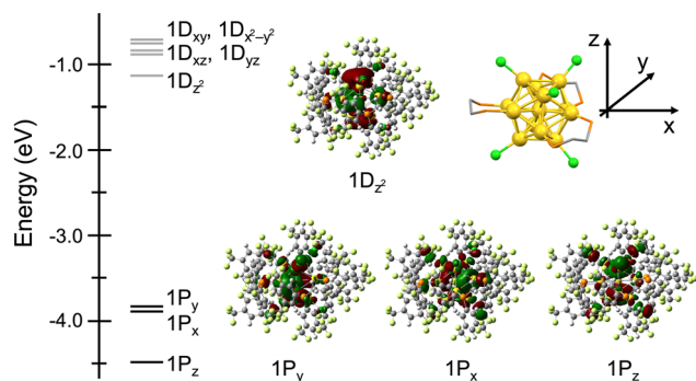
Fig. 3 Energy diagrams and KS orbitals of Au 13 :dppeF (isovalue = 0.02). The top-right figure shows the orientation of the Au 13 :dppeF NC without the \text{Ar}^{\text{F}} moieties and H atoms, which have been removed for clarity.
