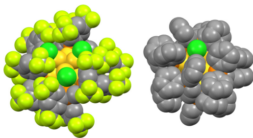
Fig. 4 Space-filling models of Au 13 :dppeF (left) and Au 13 :dppe (right) around the Cl coordination sites. Color code: Au, yellow; P, orange; Cl, green; C, gray; F, yellow-green.
