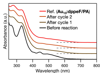
Fig. 6 UV-Vis absorption spectra of initial Au 13 :dppeF (black) and Au 13 :dppeF after cycles 1 (dark brown) and 2 (brown), along with the spectrum of Au 13 :dppeF/PA (red) as a reference.
