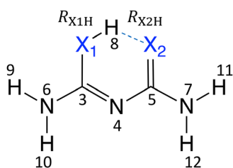
Fig. 2 Structure and definition of atomic labels and structural parameters for dithiobiuret ( X_1 and X_2 = S) and thiobiuret ( X_1 = O and X_2 = S).
