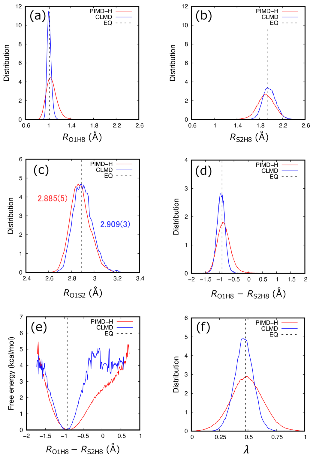
Fig. 6 One-dimensional distributions of (a) R_{O1H8} , (b) R_{S2H8} , (c) R_{O1S2} , (d) R_{O1H8} - R_{S2H8} , (e) relative free energies, and (f) \pi -delocalization index ( \lambda ) for thiobiuret obtained from PIMD and CLMD simulations.
