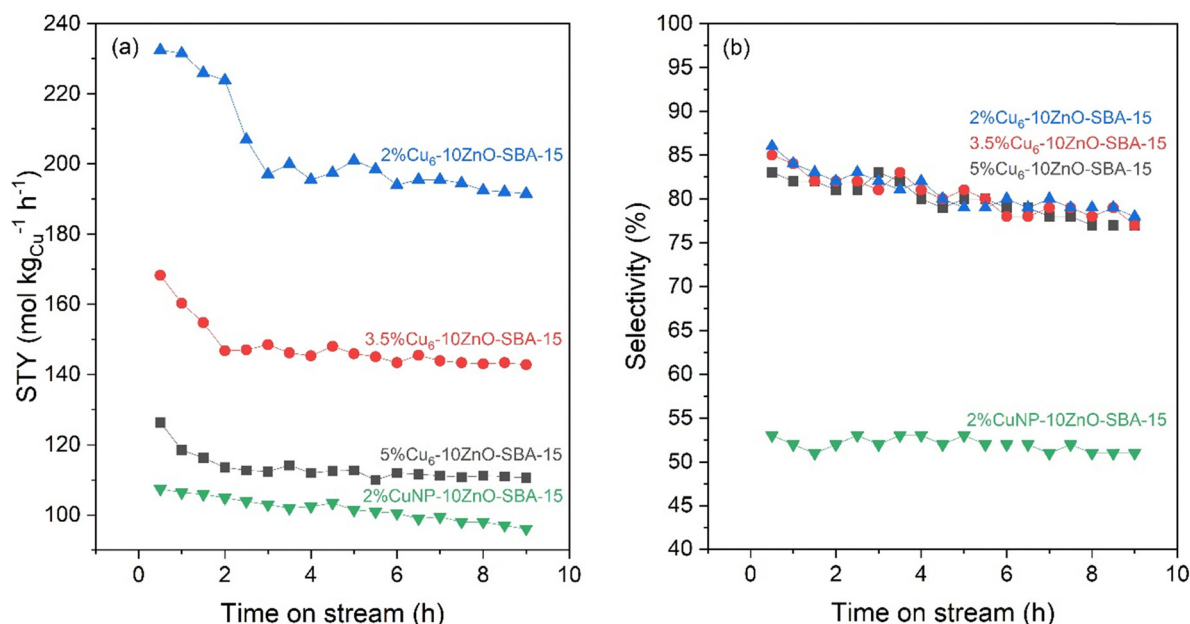
Fig. 8 (a) Space-time yield and (b) selectivity of methanol versus time-on-stream of the catalysts. Reaction conditions: T = 220 °C; P = 5.0 MPa; \text{H}_2/\text{CO}_2 = 3 \text{ mol mol}^{-1} ; \text{GHSV} = 7500 \text{ mL g}^{-1} \text{ h}^{-1} ; m_{\text{cat}} = 0.2 \text{ g} .
