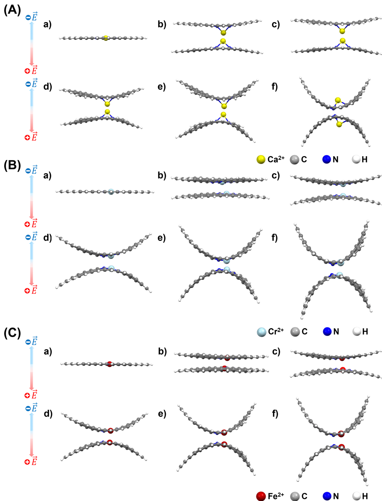
Fig. 5 Geometry optimization of the M^{2+} -4N-GQD model for (A) Ca^{2+} , (B) Cr^{2+} , and (C) Fe^{2+} under varying electric fields: (a) 0.0 a.u., (b) 0.010 a.u., (c) 0.0150 a.u., (d) 0.020 a.u., (e) 0.025 a.u., and (f) 0.030 a.u.
