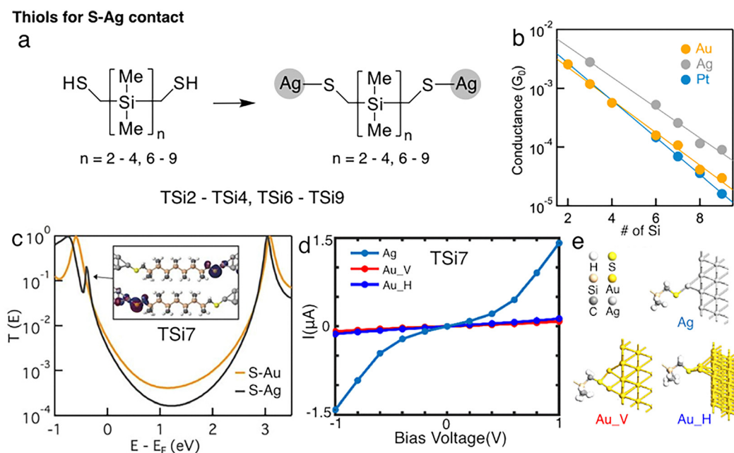
Fig. 7 (a) Chemical structures and formed molecular junctions of TSi2 – TSi4 and TSi6 – TSi9 . (b) Conductance plotted against the number of silicon atoms in the backbone for TSi2 – TSi4 and TSi6 – TSi9 measured with Au (orange), Ag (grey), and Pt (blue) electrodes, and lines showing linear fits to the data following the G = G_{\text{CE}} e^{-\beta n} equation. (c) Calculated transmission curves for Au– TSi7 –Au (orange) and Ag– TSi7 –Ag (grey) junctions. Inset: Gateway state orbitals. (d) Calculated current–voltage curves of Au– TSi7 –Au and Ag– TSi7 –Ag junctions. Two binding configurations V and H for Au– TSi7 –Au junctions are included in the calculation. (e) Optimized geometric structures of molecular junctions for the Ag(111) electrode with one protruding Ag atom surface, and Au(111) electrode with the vertical/horizontal configuration of a double atomic surface (Au_V/Au_H). (b) and (c) are adapted with permission from ref. 21, copyright (2017) Wiley-VCH. (d) and (e) are adapted with permission from ref. 96, copyright (2023) The Royal Society of Chemistry.
