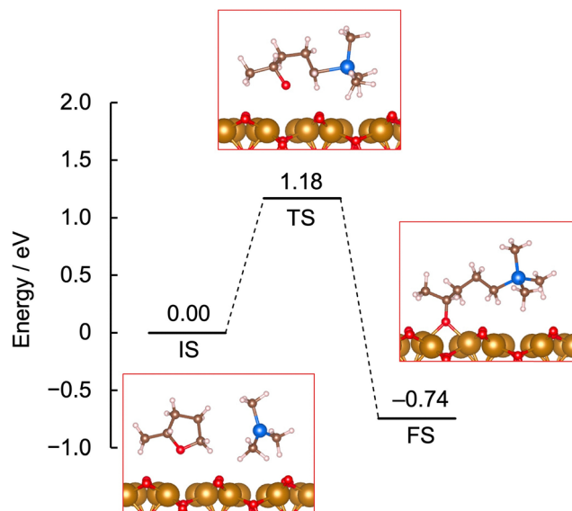
Fig. 7 Potential energy profile for cleavage of the ether \text{C}(\text{sp}^3)\text{--O} bond on the \alpha\text{-Fe}_2\text{O}_3 surface. Color coding: brown for Fe, red for O, blue for Si, white for H, and dark brown for C.
