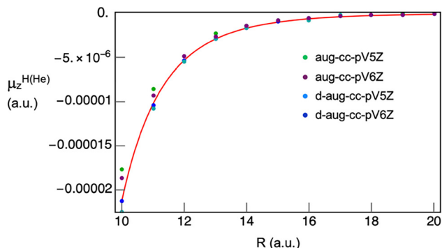
Fig. 13 DMA dispersion dipole for the H center in HeH from several different basis sets, and the prediction of long-range perturbation theory including R^{-7} , R^{-9} , and R^{-11} terms (red).
