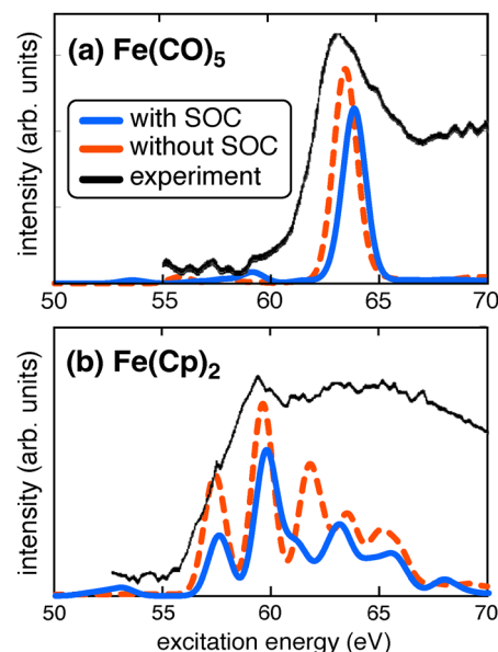
Fig. 10 XUV spectra at the Fe M-edge, comparing CAM-B3LYP/CIS simulations to experimental spectra from ref. 130. Calculations employ the def2-TZVPD basis set with 200 singlet and 200 triplet states. Transition energies were broadened using a Lorentzian function (FWHM = 0.5 eV) but have not been shifted.
