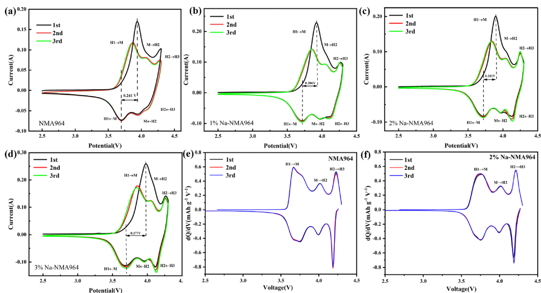
Fig. 4 Initial three CV curves of (a) NMA964, (b) 1%Na-NMA964, (c) 2%Na-NMA964, and (d) 3%Na-NMA964 with a scan rate of 0.2 \text{ mV s}^{-1} . The dQ/dV profiles of the initial three cycles for (e) NMA964 and (f) 2%Na-NMA964.
