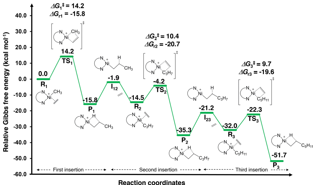
Fig. 5 The relative Gibbs free energies profile for ET polymerization catalyzed by Ni- \alpha -diimine at 6-31G(d) levels in gas phase. The activation free energy ( \Delta G^\ddagger ), and reaction energy ( \Delta G_r ) were shown in kcal mol -1 .
