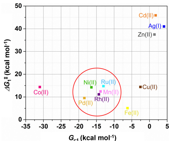
Fig. 6 The relationship between the coordination free energy ( G_{c1} ) and activation free energy ( \Delta G^\ddagger ) of M- \alpha -diimine catalysts with different metal substitutions.
