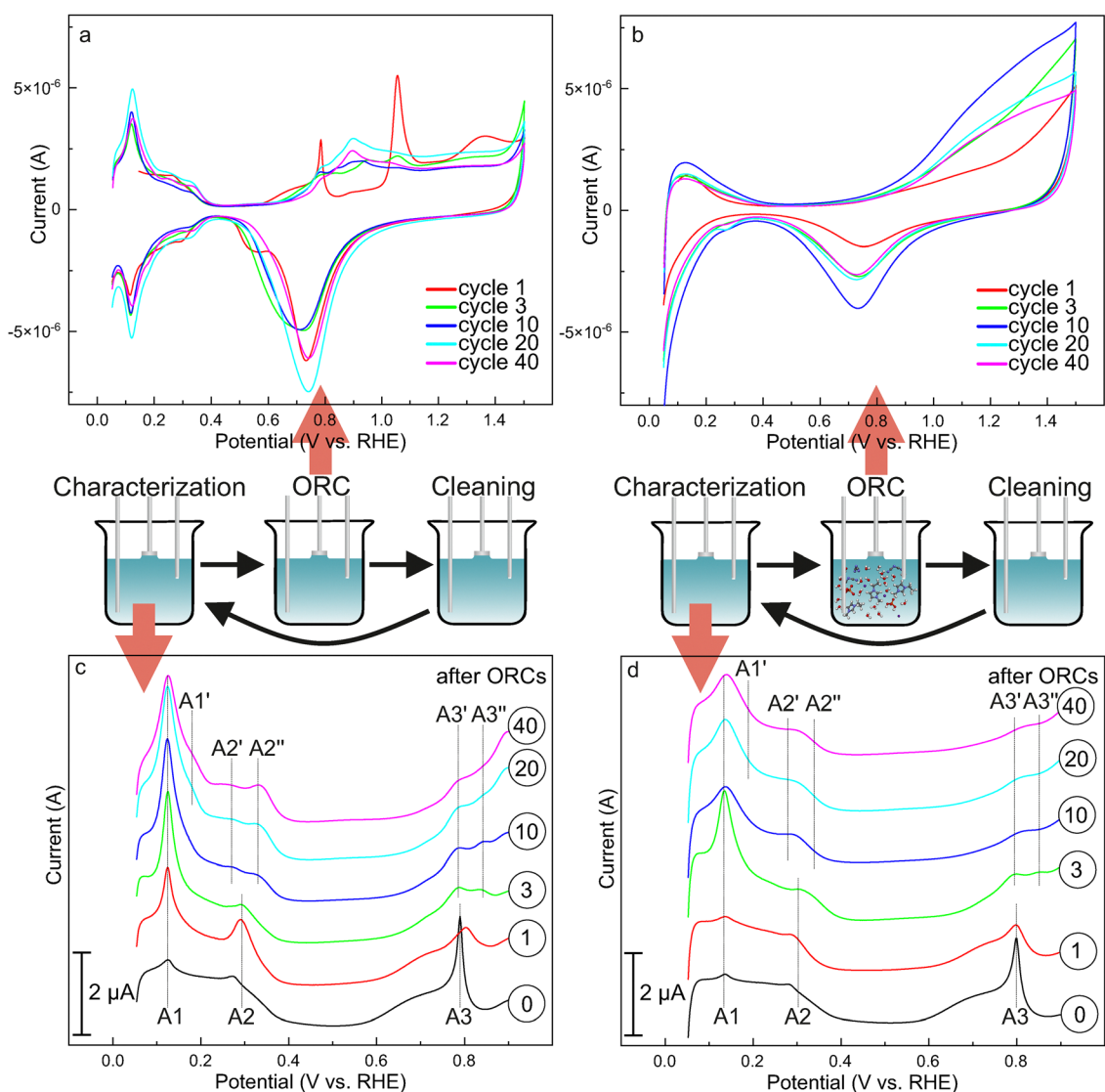
Fig. 2 Cyclic voltammograms of Pt(111) during ORCs ( 0.05\text{--}1.5\text{ V}_{\text{RHE}} , 50\text{ mV s}^{-1} ) in the absence (a) and presence (b) of 1\text{ M }[\text{C}_2\text{C}_1\text{Im}][\text{OTf}] . Corresponding characterization CVs ( 0.05\text{--}0.9\text{ V}_{\text{RHE}} , 50\text{ mV s}^{-1} ) measured after ORCs in absence (c) and presence (d) of IL in blank electrolyte only ( 0.1\text{ M HClO}_4 ). An additional cleaning step was performed between the ORCs and the characterization.
