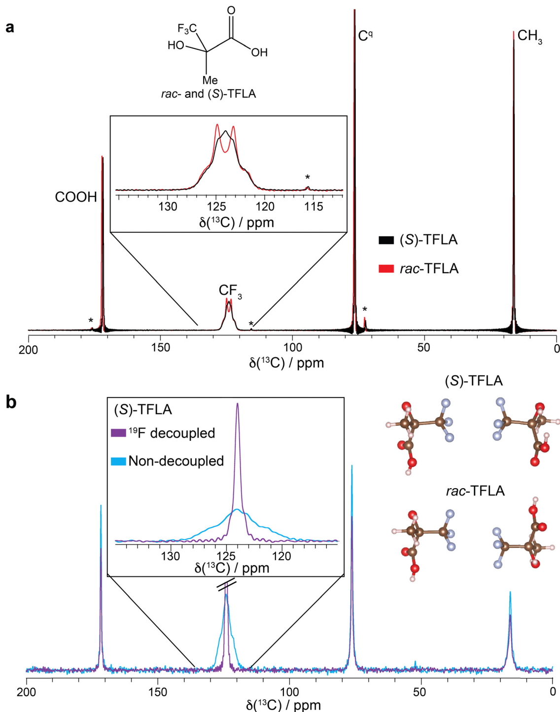
Fig. 1 (a) ^1H - ^{13}C CP spectra of ( S )- and rac -TFLA recorded at 17.5 kHz and 16.4 T static magnetic-field strength. The chemical structure of TFLA is shown. (b) ^{19}F - ^{13}C CP spectra of ( S )-TFLA recorded at 15.0 kHz and 11.7 T with and without ^{19}F high-power decoupling during data acquisition. The homochiral and heterochiral dimeric units taken from the crystal structures of ( S )- and rac -TFLA (CSD numbers: ( S )-TFLA refined from 666327 – for more details see Experimental section – and rac -TFLA 666328), respectively, are additionally shown. 20 * denotes MAS spinning sidebands. Signal truncation in a results from too short acquisition times.
