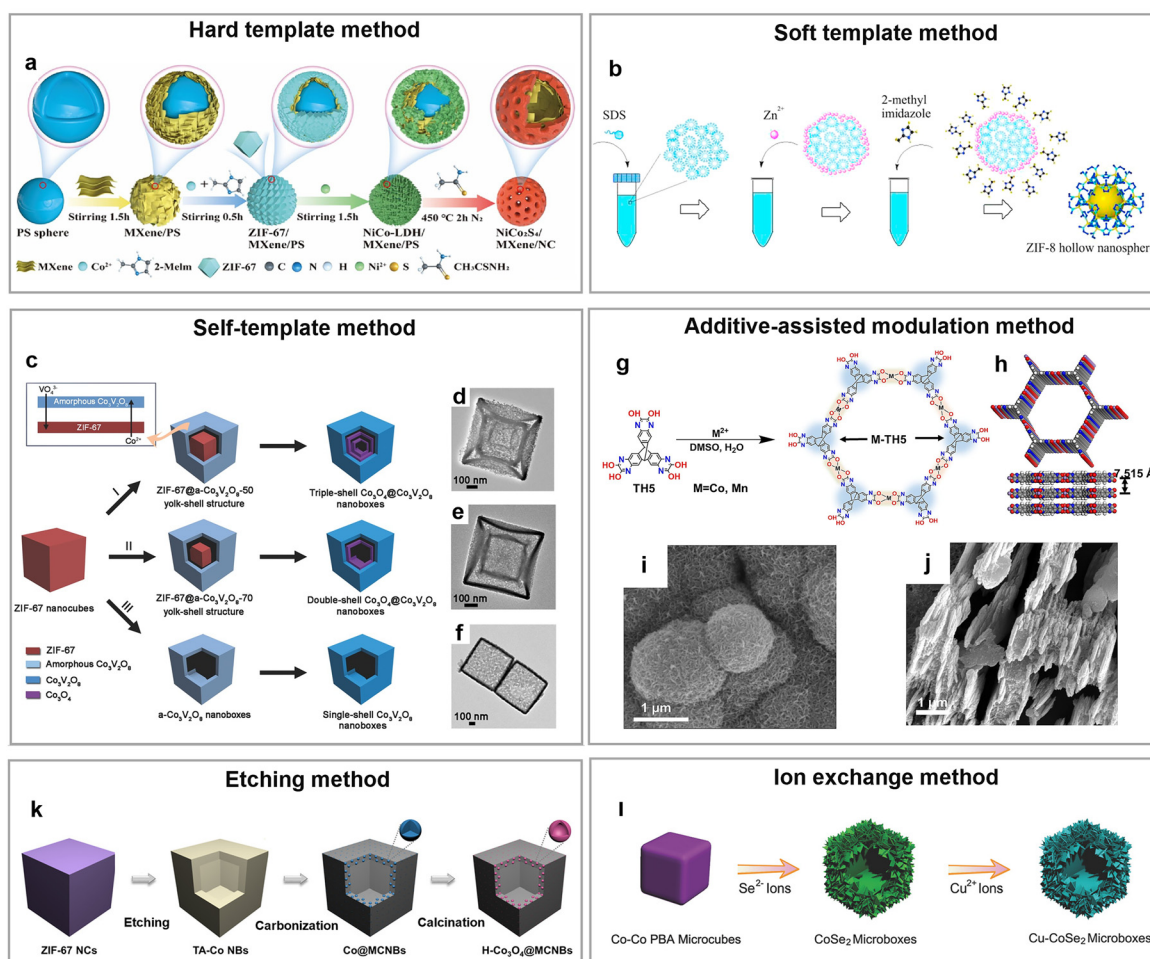
Fig. 3 Some typical synthesis strategies of hierarchical architectural structures: (a) schematic diagram of \text{NiCo}_2\text{S}_4/\text{MXene}/\text{NC} ; reproduced with permission from ref. 70. Copyright 2024, Elsevier. (b) Schematic diagram of ZIF-8 hollow nanospheres; reproduced with permission from ref. 76. Copyright 2015, Elsevier. (c) Schematic diagram of \text{Co}_3\text{O}_4@/\text{Co}_3\text{V}_2\text{O}_8 hollow structures; (d–f) TEM images of the corresponding products; reproduced with permission from ref. 78. Copyright 2017, WILEY-VCH. (g) Synthetic diagram of M-TH5; (h) 3D view of M-TH5; (i) SEM image of Mn-TH5; (j) SEM image of Co-TH5; reproduced with permission from ref. 80. Copyright 2024, Elsevier. (k) Schematic diagram of the formation process of \text{H-Co}_3\text{O}_4@/\text{MCNBs} ; reproduced with permission from ref. 82. Copyright 2020, Wiley-VCH. (l) Schematic illustration of the synthesis of \text{Cu-CoSe}_2 microboxes; reproduced with permission from ref. 84. Copyright 2018, Wiley-VCH.
