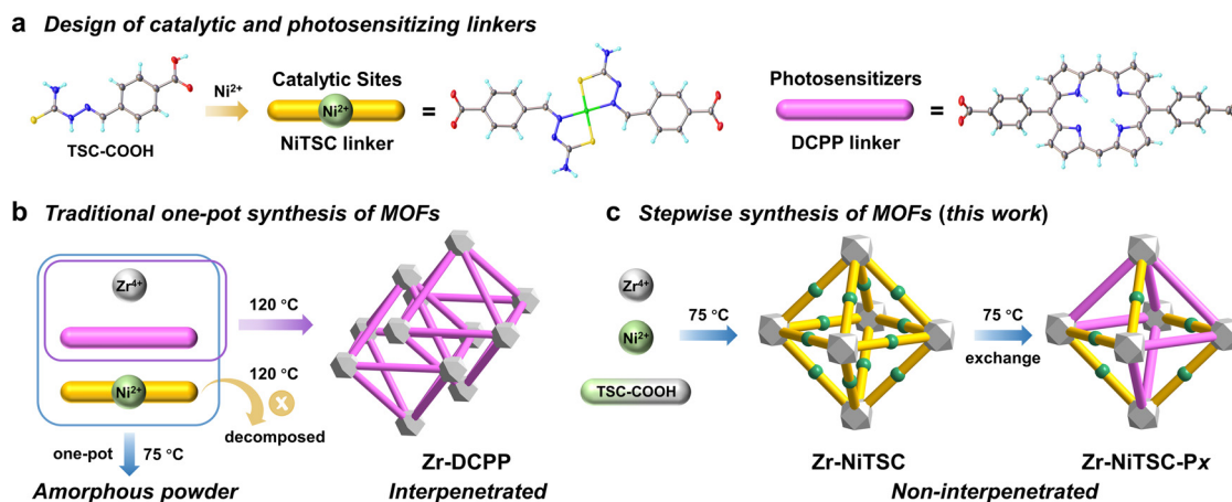
Fig. 1 (a) Design and single-crystal structures of NiTSC and DCPP linkers (green: Ni; yellow: S; blue: N; gray: C; red: O; light blue: H). Schematic diagram of the (b) traditional one-pot synthesis and (c) stepwise synthesis of Zr-NiTSC-P x (P stands for porphyrin, x = 1, 2, or 3).
