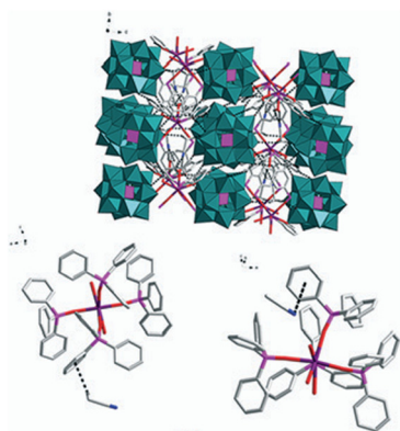
Fig. 8 The crystal stacking of complex [Nd(TPPO) 4 (H 2 O) 3 ](PMO 12 O 40 )·4CH 3 CN.
