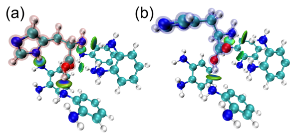
Fig. 2 The isosurface IGM figure of the optimized complexes of 1,2-diaminobenzene and (a) L- or (b) D-His at a 4:1 molar ratio. The blueish-green ellipsoid areas indicate non-covalent interactions.
