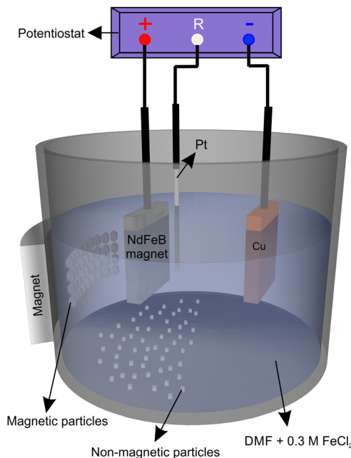
Fig. 8 Schematic illustration of the electrolytic cell for recovering the Nd 2 Fe 14 B grains from the sintered NdFeB magnets. Reproduced with permission from ref. 11.
