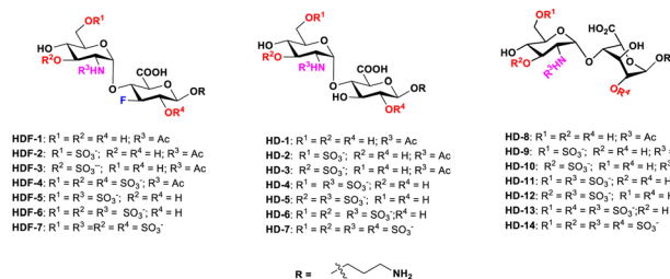
Fig. 1 Chemical structures of 7-fluorinated D-glucuronic acid based HS mimetics (HDF-1 to HDF-7) and 14 native HS disaccharides (D-glucuronic acid based HD-1 to HD-7 and L-iduronic acid based HD-8 to HD-14).
