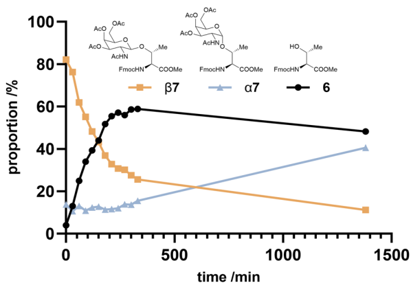
Fig. 2 Product distribution over time following treatment of a 7 : 1 \beta 7/ \alpha 7 mixture to 1 equiv. Cu(OTf) 2 in refluxing DCE as determined by LCMS (UV absorbance at 280 nm).
