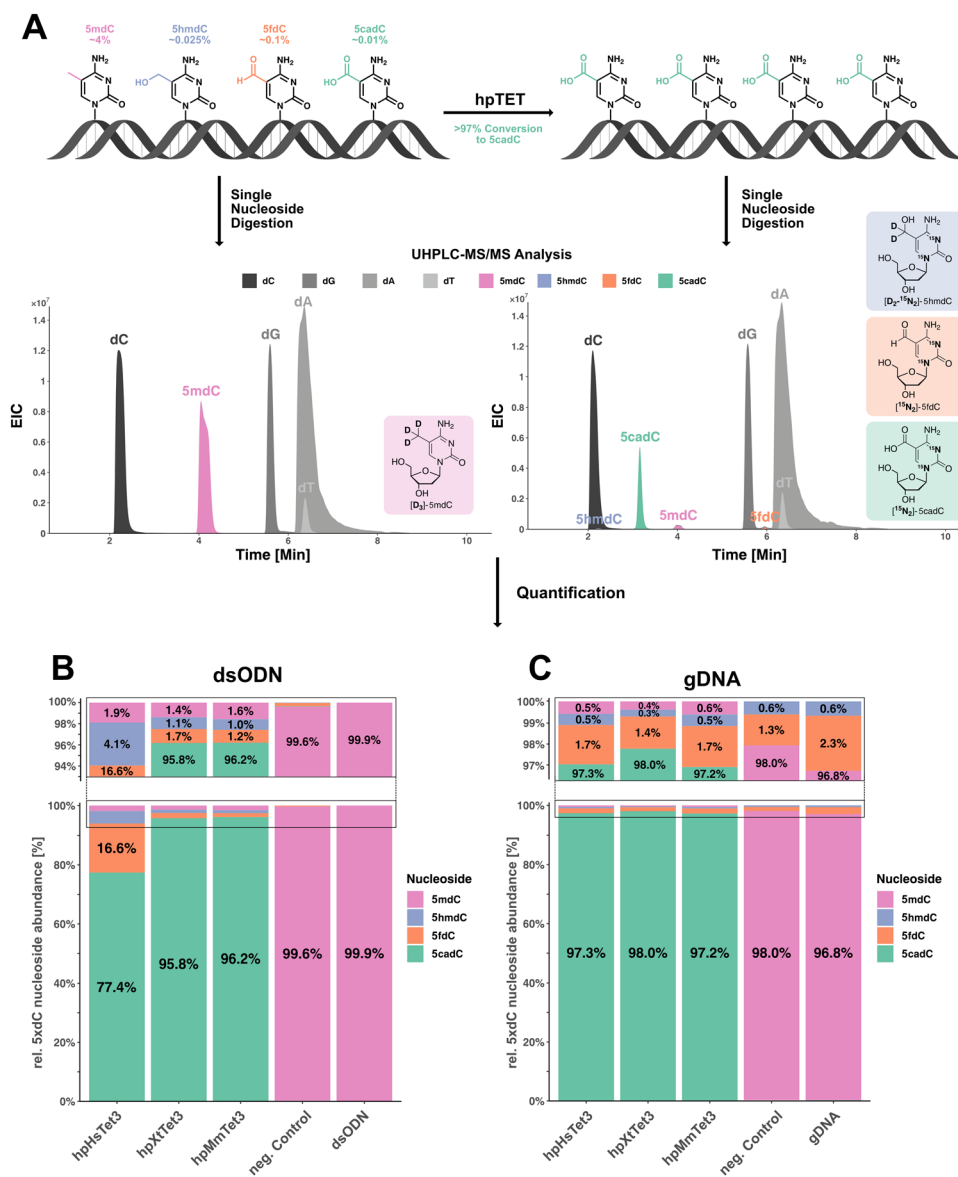
Fig. 3 Oxidation of 5mxC by hpTet3-enzymes in synthetic and genomic DNA. (A) Principle of the LC-MS/MS-based quantification of 5mxC, 5hmdC, 5f dC, and 5cadC in hpTet3-treated dsODN/gDNA samples and structures of used isotopologues. (B) Plot of the relative percentage of the quantified modified cytidines in the double-stranded 35-mer and (C) HEK293T gDNA following enzymatic treatment. gDNA: isolated gDNA was digested, and dC and modified dC nucleosides were quantified. As a negative control, ODN or gDNA were incubated under Tet-oxidation conditions, but without the addition of hpTet-enzymes, followed by digestion and quantification.
