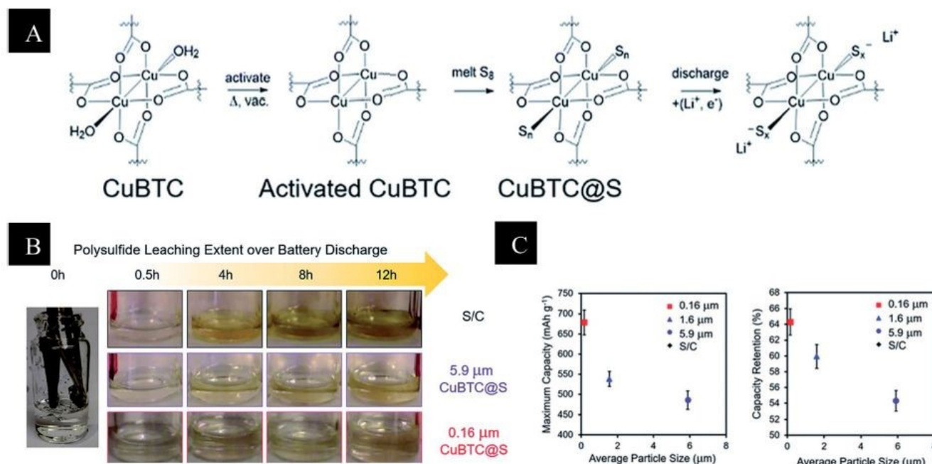
13 Fig. 7 (A) Activation and sulfur loading of HKUST-1 with potential binding sites at the Cu 14 paddlewheel. (B) Electrolyte samples of 0.16 \mu\text{m} and 5.9 \mu\text{m} CuBTC, and S/C electrodes during 15 a galvanostatic discharge of C/20. Yellow discoloration indicates the amount of leached 16
