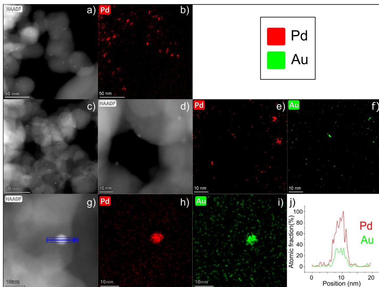
Figure 2: (a) HAADF-STEM image of Pd/C and (b) the relative EDX of Pd distribution. (c-d) HAADF-STEM images of Au-Pd/C and (e-f) EDX analysis for Pd and Au of the region shown in f. (g) HAADF-STEM image of a single
