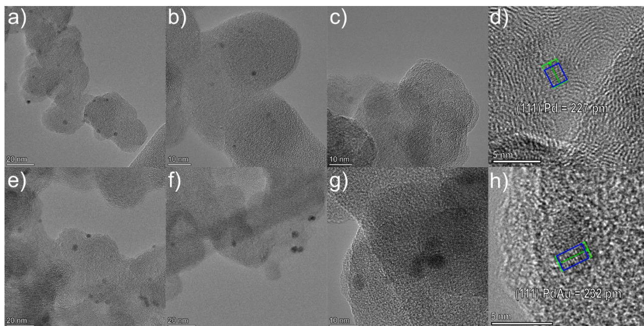
Figure 1: HR-TEM images of (a-c) Pd/C and (e-g) PdAu/C and measured lattice spacings of an individual Pd NP (d) and an individual PdAu NP (h).
