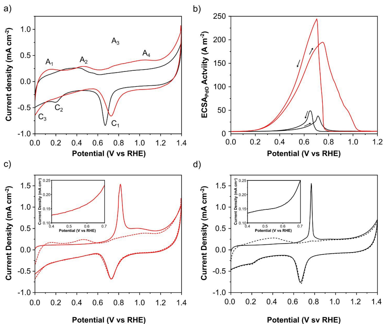
Figure 3: Electrochemical characterization (a) CVs of PdAu/C (red) and Pd/C (black) (N 2 saturated 2M KOH; 0 to 1.4 V (RHE) scan rate 50 mV s -1 ); (b) in N 2 saturated 2 M HCOOK and 2 M KOH (0 to 1.2 V (RHE) at a scan rate 50 mV s -1 ). CO ads stripping curves (full curves) and CVs after CO ads stripping (dashed curves) both at 20 mV s -1 for (c) PdAu/C and (d) Pd/C respectively. The inserts within Figures (c) and (d) show a zoom on the onset region of CO oxidation.
