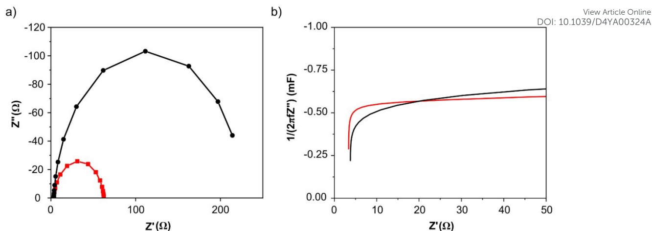
Figure 4. Electrochemical impedance spectroscopy (EIS) of PdAu/C (red curves) and Pd/C (black curves) in KOH 2M at 0.4V vs RHE: a) Nyquist plot and b) Capacitance plot.
