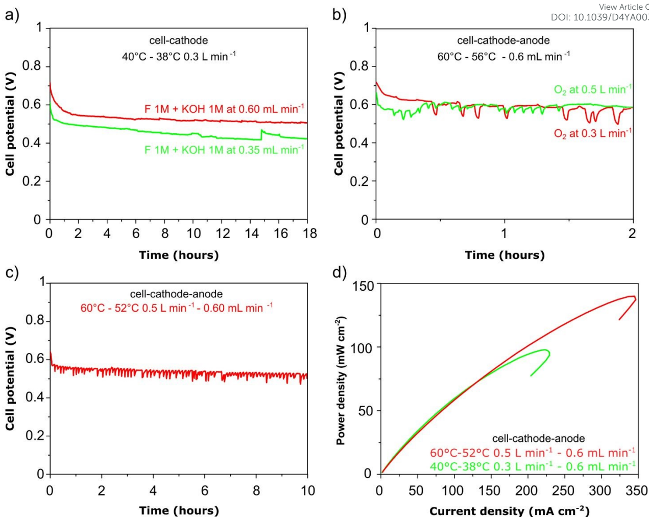
Figure 6: DFFC stability experiments carried out a single pass fuel feed (galvanostatic – 0.05 A cm -2 ). (a) variable anode flow; (b) variable cathode flow; (c) high anode and high cathode flow test showing stable power density delivery; (d) Power density vs current density curves at variable cell temperature. All experiments fuel composition 1 M KOH and 1 M HCOOK.
