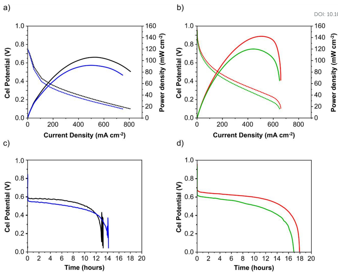
Figure 5. Direct formate fuel cell experiments containing the Pd/C (a and c) and PdAu/C anode (b and d). All cells used FeCo/C cathode catalyst and Fumatech FAA-3-30 AEM. The fuel was 1 M HCOOK and 1 M KOH. T_{\text{cell}} 60 °C: Figures (a) and (b) are voltage and power density curves. Figures (c) and (d) are cell voltage at constant current density 0.05 A cm -2 . First and fifth cycle for Pd/C are respectively black and blue curves, while for PdAu/C are red and green.
