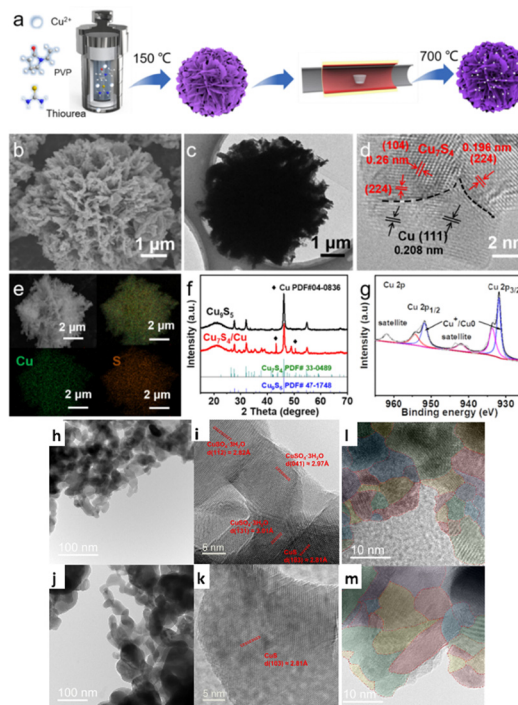
Fig. 10 (a) Schematic illustration of the synthetic process, (b) SEM image, (c) TEM image, (d) HRTEM image, (e) EDS elemental mapping, and (g) XPS pattern of \text{Cu}_7\text{S}_4/\text{Cu} . (f) XRD patterns of \text{Cu}_7\text{S}_4/\text{Cu} and \text{Cu}_9\text{S}_5 (reproduced with permission from ref. 134, copyright Wiley-VCH 2024). Morphological and structural characterization of CuS 811 and CuS MKL before \text{ECO}_2\text{R} by electron imaging. (h) and (i) Aberration-corrected TEM images of (h) CuS 811 and (i) CuS MKL. (j) and (k) HRTEM images of (j) CuS 811 and (k) CuS MKL. The crystal facets with heterogeneous species are highlighted in (j) and (k). Structural characterisation of CuS 811 and CuS MKL post \text{ECO}_2\text{R} by electron imaging. (l) and (m) HRTEM images of (l) CuS 811 and (m) CuS MKL. Red dash-dotted lines highlight the boundaries of induced grains, and the grains with heterogeneous lattice fringes are marked in various colours (l) and (m). The marking colours are only used to distinguish every grain, and there is no correlation between the colour and phase (reproduced with permission from ref. 135, copyright Wiley-VCH 2024).
