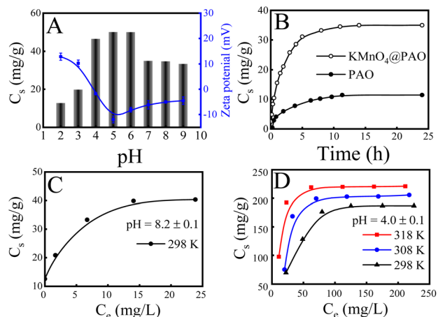
Fig. 4 Effect of pH on zeta potential of \text{KMnO}_4@\text{PAO} for \text{U}(\text{vi}) (A); effect of pH (A) and contact time on adsorption capability of \text{KMnO}_4@\text{PAO} and on PAO at \text{pH} = 8.2 \pm 0.1 (B); adsorption isotherms of \text{U}(\text{vi}) on \text{KMnO}_4@\text{PAO} and on PAO at \text{pH} = 8.2 \pm 0.1 (C) and at \text{pH} = 4.0 \pm 0.1 (D). m/V = 0.4\text{ g L}^{-1} , I = 0.1\text{ mol per L NaCl} . (A) T = 298 \pm 1\text{ K} , contact time: 24 h, C[\text{U}(\text{vi})]_{\text{initial}} = 20\text{ mg L}^{-1} , \text{pH} = 8.2 \pm 0.1 . (B) T = 298 \pm 1\text{ K} , C[\text{U}(\text{vi})]_{\text{initial}} = 20\text{ mg L}^{-1} , \text{pH} = 8.2 \pm 0.1 . (C) T = 298\text{ K} \pm 1\text{ K} , contact time: 24 h, \text{pH} = 8.2 \pm 0.1 . (D) Contact time: 24 h, \text{pH} = 4.0 \pm 0.1 .
