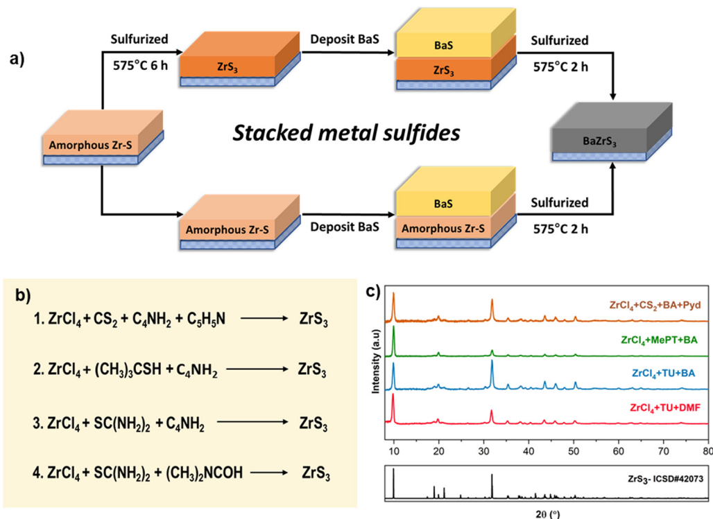
Fig. 2 (a) Reaction schematic depicting the synthesis of \text{BaZrS}_3 by layering binary sulfides. (b) Various molecular precursor chemistries employed for depositing \text{ZrS}_3 film. (c) Plot comparing the X-ray diffraction patterns of \text{ZrS}_3 film prepared using different solution chemistries, (i) \text{ZrCl}_4 + thiourea (TU) + dimethyl formamide (DMF), (ii) \text{ZrCl}_4 + TU + butylamine (BA), (iii) \text{ZrCl}_4 + 2-methyl-2-propanethiol (MePT) + BA and (iv) \text{ZrCl}_4 + BA + \text{CS}_2 + pyridine (Pyd).
