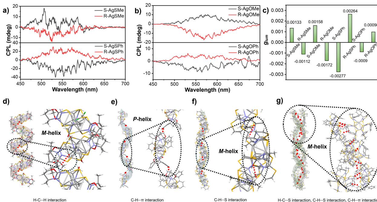
Fig. 5 (a) CPL spectra of R/S -AgSMe and R/S -AgSPh in EtOH suspension, (b) CPL spectra of R/S -AgOMe in EtOH suspension and R/S -AgOPh in MeOH suspension, (c) g_{lum} factors of various clusters detected in (a) and (b), (d) H–C⋯H interaction-driven left-handed ( M ) helical stacking of the R -AgOMe cluster in a single-crystal structure, (e) C–H⋯ \pi interaction-driven right-handed ( P ) helical stacking of the R -AgOPh cluster in a single-crystal structure, (f) C–H⋯S interaction-driven left-handed ( M ) helical stacking of the R -AgSMe cluster in a single-crystal structure, and (g) H–C⋯S interaction-, H–C⋯S interaction- and C–H⋯ \pi interaction-driven left-handed ( M ) double helix of the S -AgSPh cluster in the single-crystal structure.
