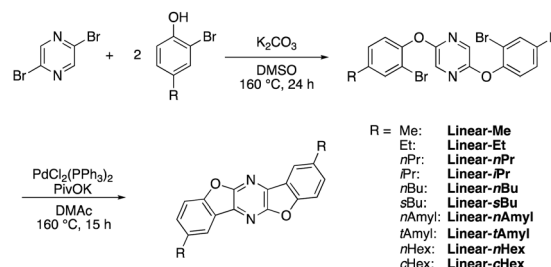
Scheme 2 Synthetic routes to linear-type bisbenzofuropyrzines.
