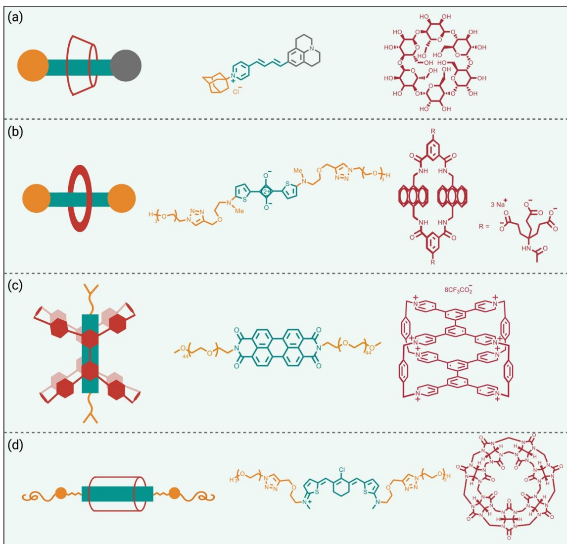
Scheme 5. Fluorophore protection by non-covalent encapsulation. The chemical structures within each panel are, ( left ) fluorophore/host complex, ( middle ) encapsulated fluorophore component, ( right ) surrounding macrocyclic host component.
