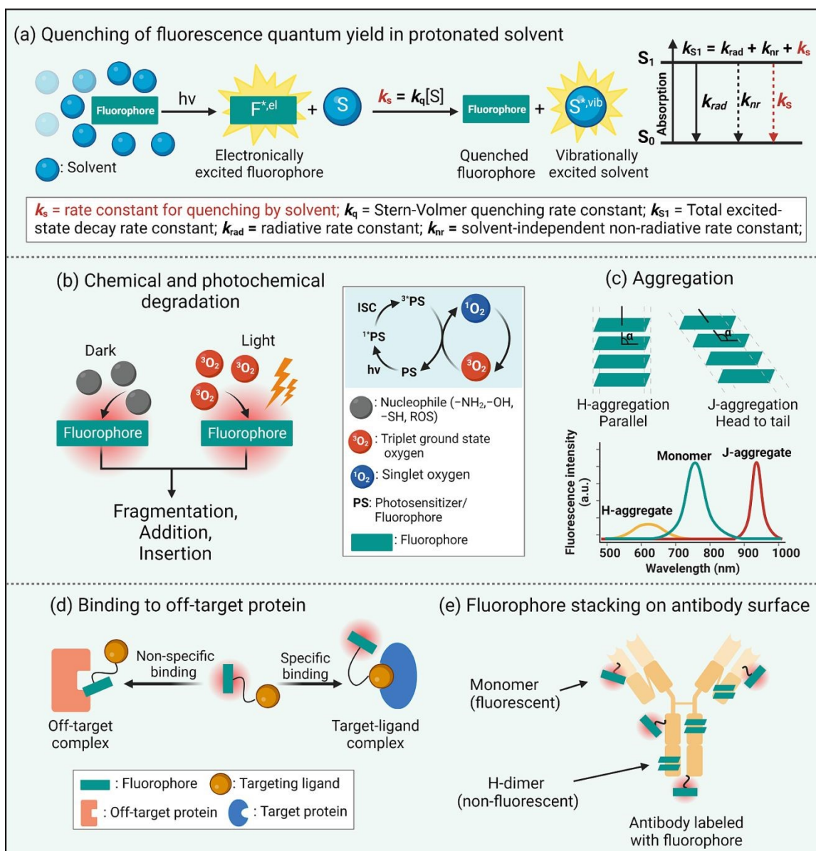
Scheme 2. Limitations of long-wavelength fluorophores.
