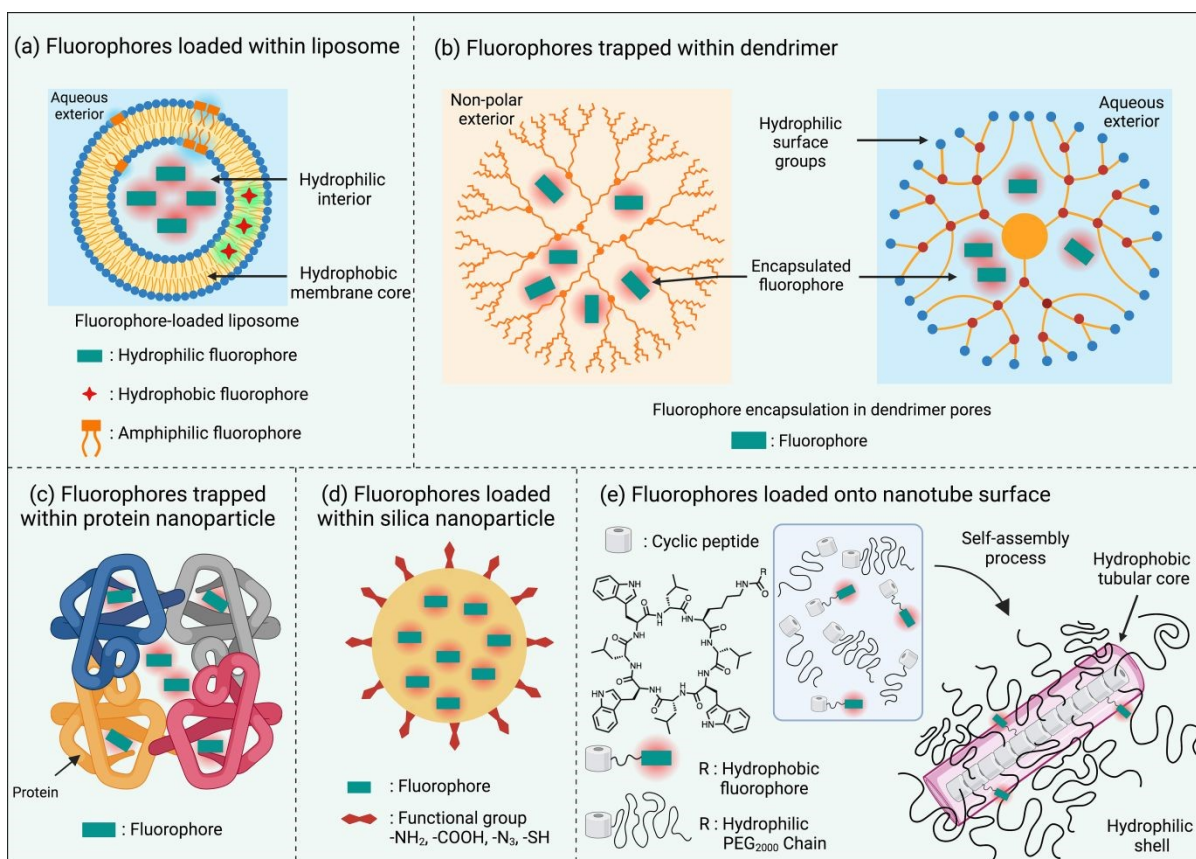
Scheme 4. Fluorophore encapsulation and protection by nanoparticles.
