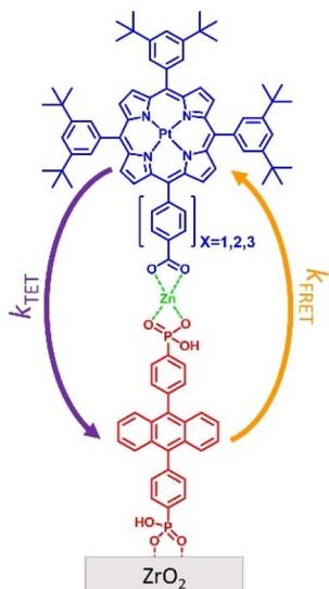
Fig. 1 General depiction of a metal ion linked bilayer composed of a \text{ZrO}_2 substrate, A (red), \text{Zn(II)} linking ion (green), and PX (blue) where X is the number of phenylene spacers. The directionality and rate constant for TET and FRET are depicted in purple and orange, respectively.
