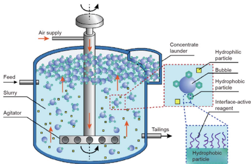
Fig. 13 Schematic of a flotation cell for hydrophobic and hydrophilic material separation. 143 Reproduced with permission from Elsevier.
