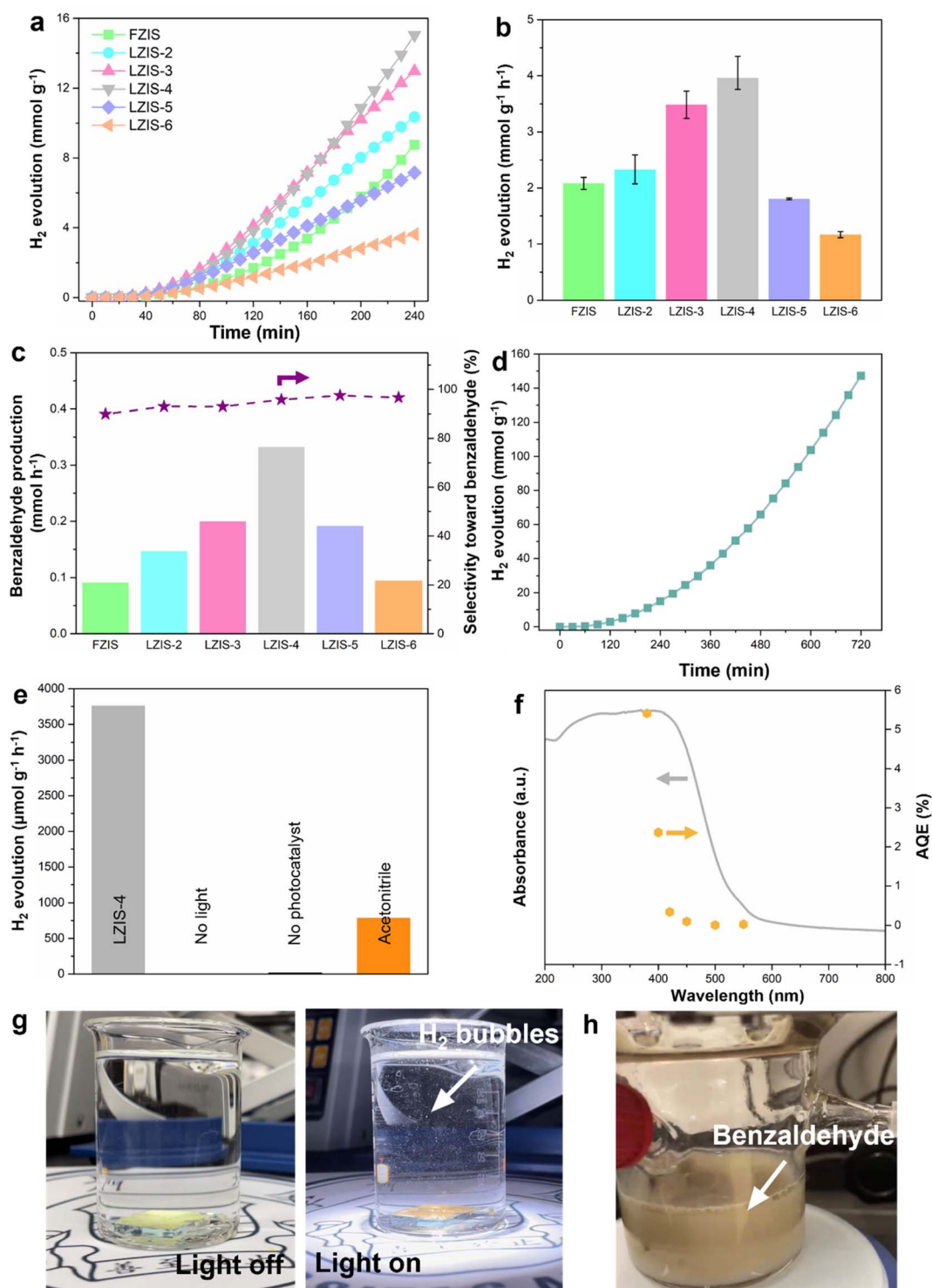
Fig. 4 (a) Time-dependent photocatalytic \text{H}_2 evolution and (b) average \text{H}_2 evolution rate over \text{ZnIn}_2\text{S}_4 samples under AM 1.5 light irradiation. (c) Benzyl alcohol conversion and selectivity toward benzaldehyde formation over all the \text{ZnIn}_2\text{S}_4 samples. (d) Prolonged stability run of 12 h for LZIS-4. (e) Control experiments using LZIS-4. (f) Apparent quantum efficiency (AQE) test of LZIS-4 at different wavelengths. (g) Digital photographs of \text{H}_2 evolution using LZIS-4 coated thin film without and with light irradiation. (h) Digital photograph of color changes of reaction medium after a 12 h dual-redox photocatalytic run with LZIS-4 as the photocatalyst.
