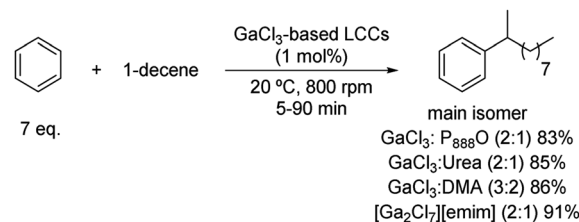
Scheme 5 Alkylation of benzene using 1-decene in GaCl 3 -based liquid coordination complexes.
