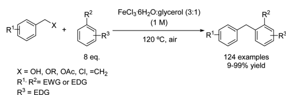
Scheme 6 FeCl 3 /glycerol promoted synthesis of diaryllkanes.
