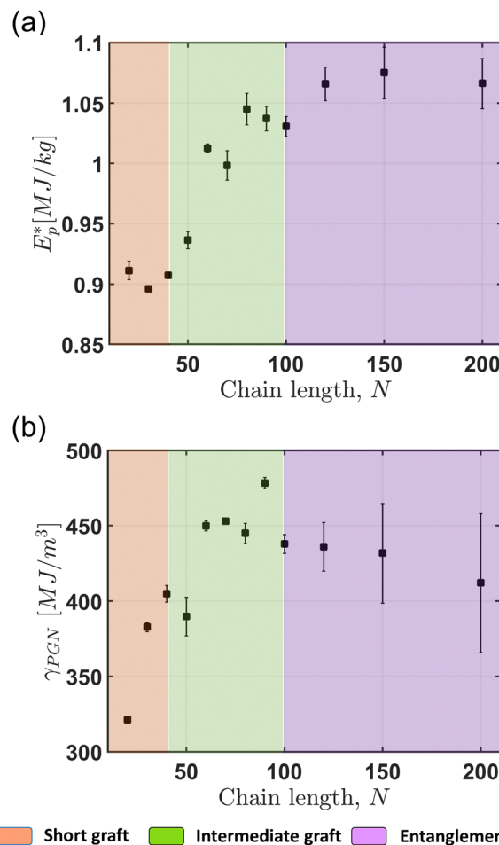
Fig. 4 (a) Specific penetration energy ( E_p^* ), and (b) cohesive energy density ( \gamma_{\text{PGN}} ) for \text{Fe}_3\text{O}_4 NP core PGNs. The E_p^* and \gamma_{\text{PGN}} are divided into three different regimes: (i) short graft, (ii) intermediate graft, and (iii) entangled graft. The error bar represents the standard deviation from three different trials.
