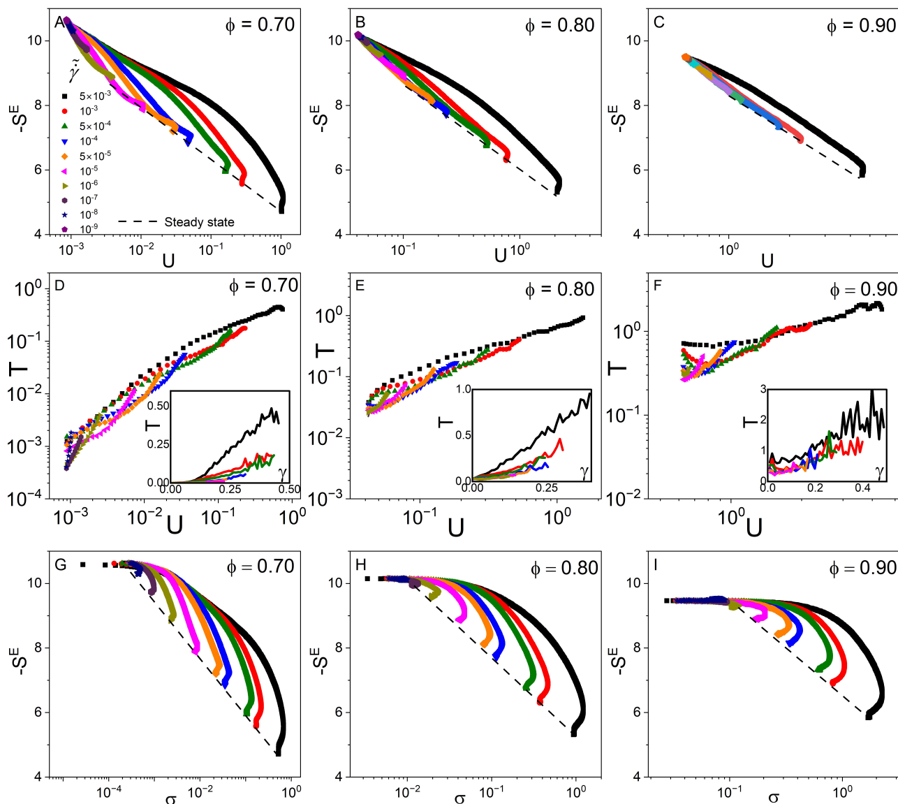
Fig. 8 Excess entropy, -S^E , (top row) and transient temperature, T , (middle row) as a function of the elastic energy, U , for suspensions with volume fraction of (A, D) \phi = 0.70 , (B, E) \phi = 0.80 , and (C, F) \phi = 0.90 . Insets are temperature as a function of strain, \gamma . Excess entropy, -S^E , (bottom row) as a function of shear stress, \sigma , at different shear rates for suspensions with volume fraction of (G) \phi = 0.70 , (H) \phi = 0.80 , and (I) \phi = 0.90 . The color-coding in all sub-figures is the same as (A).
