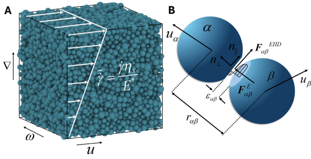
Fig. 1 (A) Configuration of suspensions with volume fraction of \phi = 0.80 in a cubic simulation box that is in the shear flow with an applied shear rate of \dot{\gamma} = \dot{\gamma}\eta_s/E^* , where E^* is the particle contact modulus and \eta_s is the suspending fluid viscosity. The flow ( \mathbf{u} ), gradient ( \nabla ), and vorticity ( \boldsymbol{\omega} = \nabla \times \mathbf{u} ) directions are shown. (B) Two particles form flat facet at a contact and interact via generalized Hertzian contact and elastohydrodynamic lubrication forces. 3
