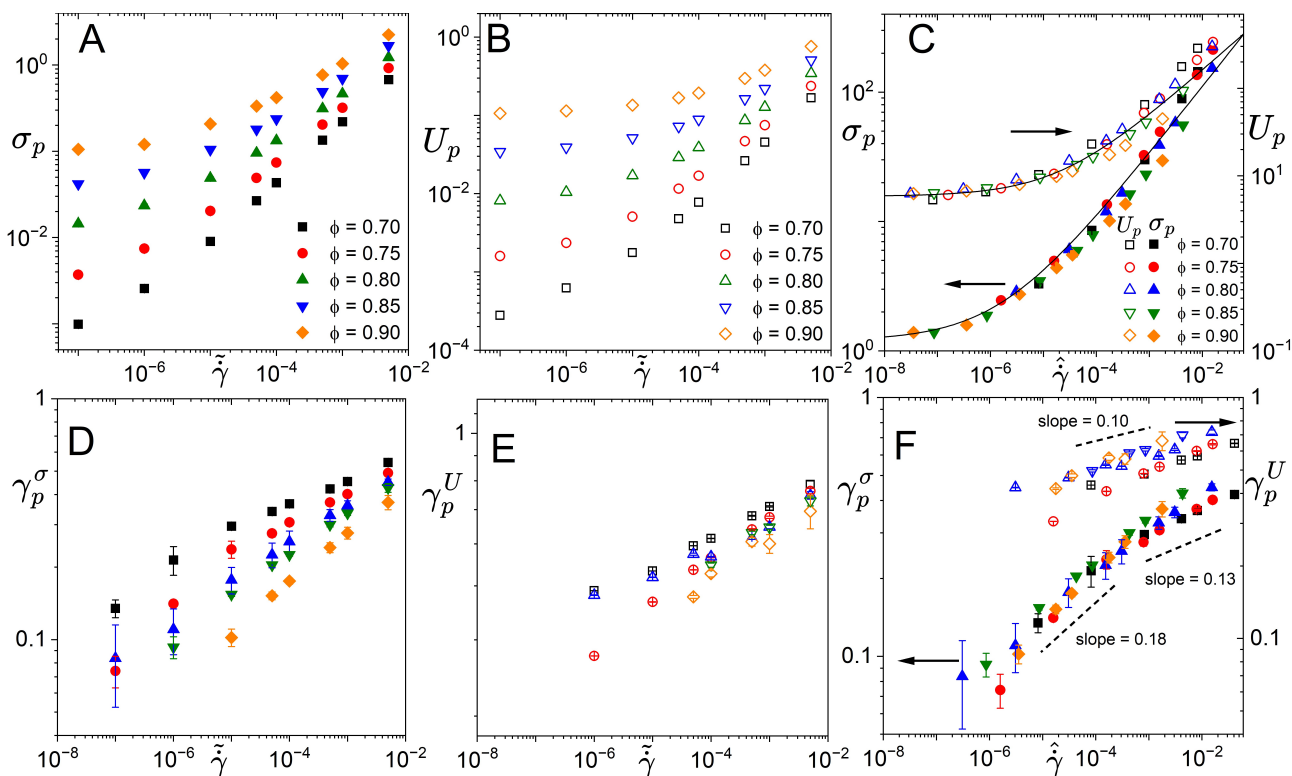
Fig. 3 (A) Peak stress, \sigma_p , and (B) peak elastic energy, U_p , as a function of the shear rate \tilde{\gamma} . (C) Master curve of the \sigma_p/\sigma_y (left axis) and U_p/U_y (right axis) as a function of the rescaled shear rate, \tilde{\gamma} , at different volume fractions. The solid lines are the HB fits to data. (D) Strain corresponding to peak stress, \gamma_p^\sigma , and (E) elastic energy, \gamma_p^U , as a function of the shear rate, \tilde{\gamma} . (F) Master curves of \gamma_p^\sigma (left axis) and \gamma_p^U (right axis) as a function of the rescaled shear rate, \tilde{\gamma} . The color-coding in (D-F), is the same as (A-C), respectively.
