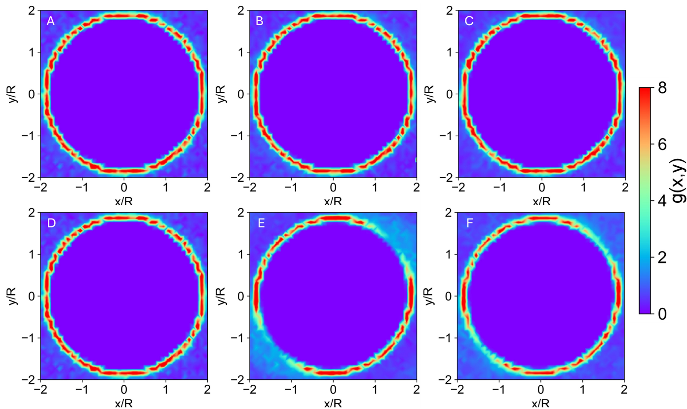
Fig. 4 Two dimensional pair distribution function, g(x,y) , at shear rate of (A-C) \dot{\gamma} = 10^{-9} and (D-F) \dot{\gamma} = 10^{-4} for \phi = 0.80 at different strains: (A, D) \gamma = 0 , (B, E) \gamma = \gamma_p^\sigma , and (C, F) \gamma = \gamma_{st} .
