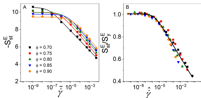
Fig. 7 Steady state excess entropy, -S^E_{st} , as a function of shear rate, \hat{\gamma} , and (B) rescaled excess entropy S^E_{st}/S^E_{st} , where S^E_{st} is the excess entropy in the dynamic yield point, as a function of the rescaled shear rate, \hat{\gamma} . The solid line shows the logarithmic fit to the data.
