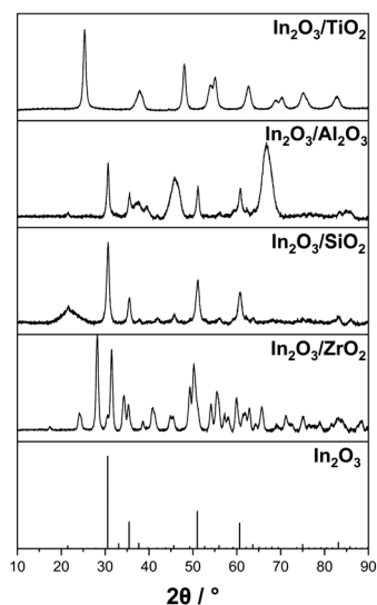
Fig. 1 X-ray diffraction measurements of self-synthesized \text{In}_2\text{O}_3 on different metal oxide supports with 6 wt% indium content and the reference diffractogram of pure \text{In}_2\text{O}_3 .
