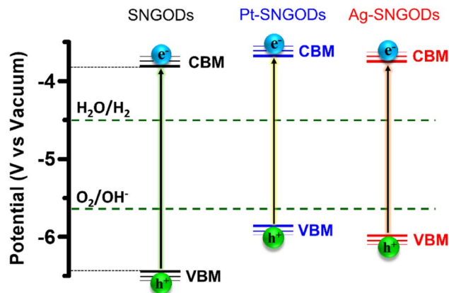
Fig. 2 Electronic-energy level diagrams of the SNGODs, Pt-SNGODs, and Ag-SNGODs in relation to the levels for H 2 and O 2 evolution reactions (HER and OER) in an aqueous solution of pH = 9.
